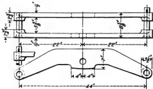
Figs. 1664-1665. Driving Box Equalizer.
